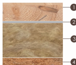
Floor insulation
