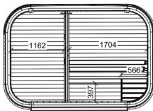
Cut view
